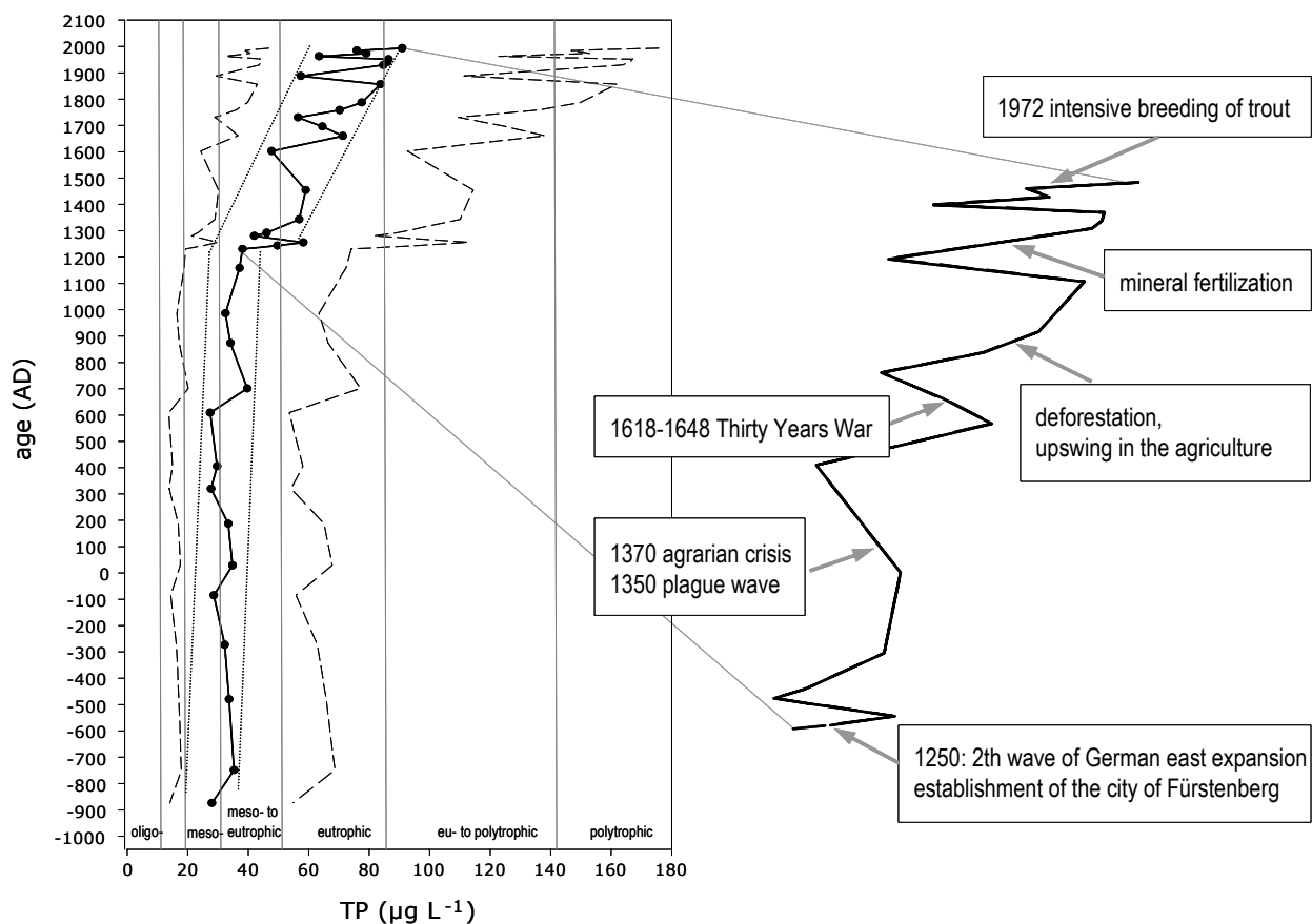
Figure 1. Long term changes of TP concentration of the lake Großer Treppelsees based on diatoms and the main historical events in the catchment which led to higher or lower TP concentrations. The strong anthropogenic impact in this flushed lake started in 1250. To reconstruct undisturbed conditions in such lake types with a large catchment area the water authorities require a quantitative look on past centuries.
