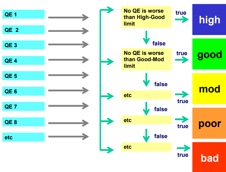
Figure 1: Representation of the WFDs classification scheme for ecological status. The ecological potential classification scheme for HMWBs and AWBs operates according to the same principles. Note that the number of relevant elements (e.g. benthic invertebrates, specific pollutants, etc) depends on (a) the status class (see Section 2 of the main guidance document); and (b) factors such as the number of specific pollutants being discharged in significant quantities.
